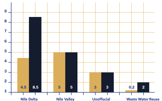
Water Resources in Egypt ( 109 m 3 /Year )
