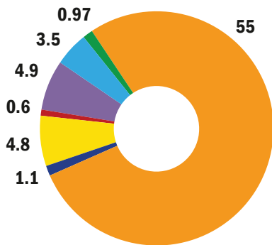
Water Resources in Egypt in Billion Cubic Meters
