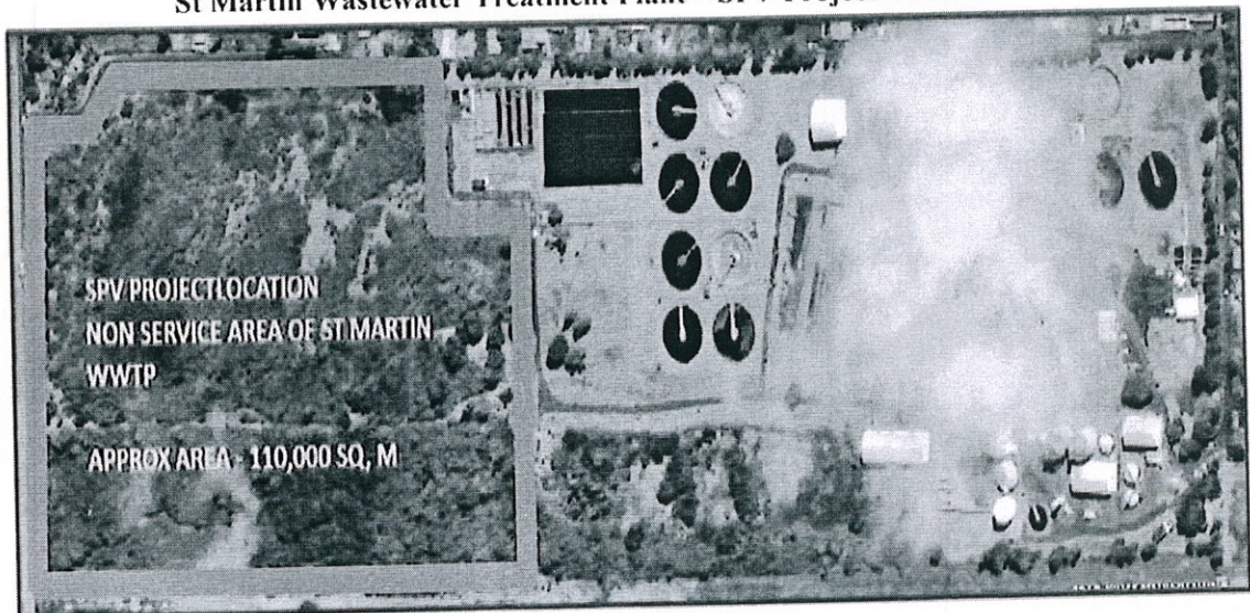
St Martin Wastewater Treatment Plant – SPV Project Location
